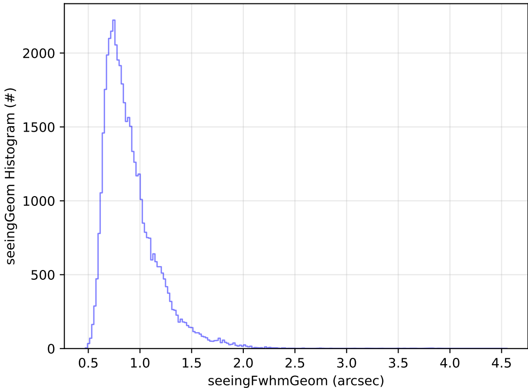
start_date_do90v3.4_10yrs Yr 1 z band: seeingGeom Histogram
