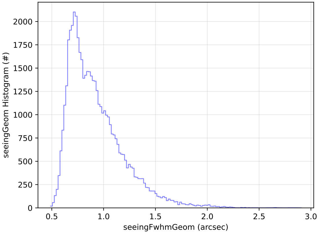
start_date_do90v3.4_10yrs Yr 1 r band: seeingGeom Histogram
