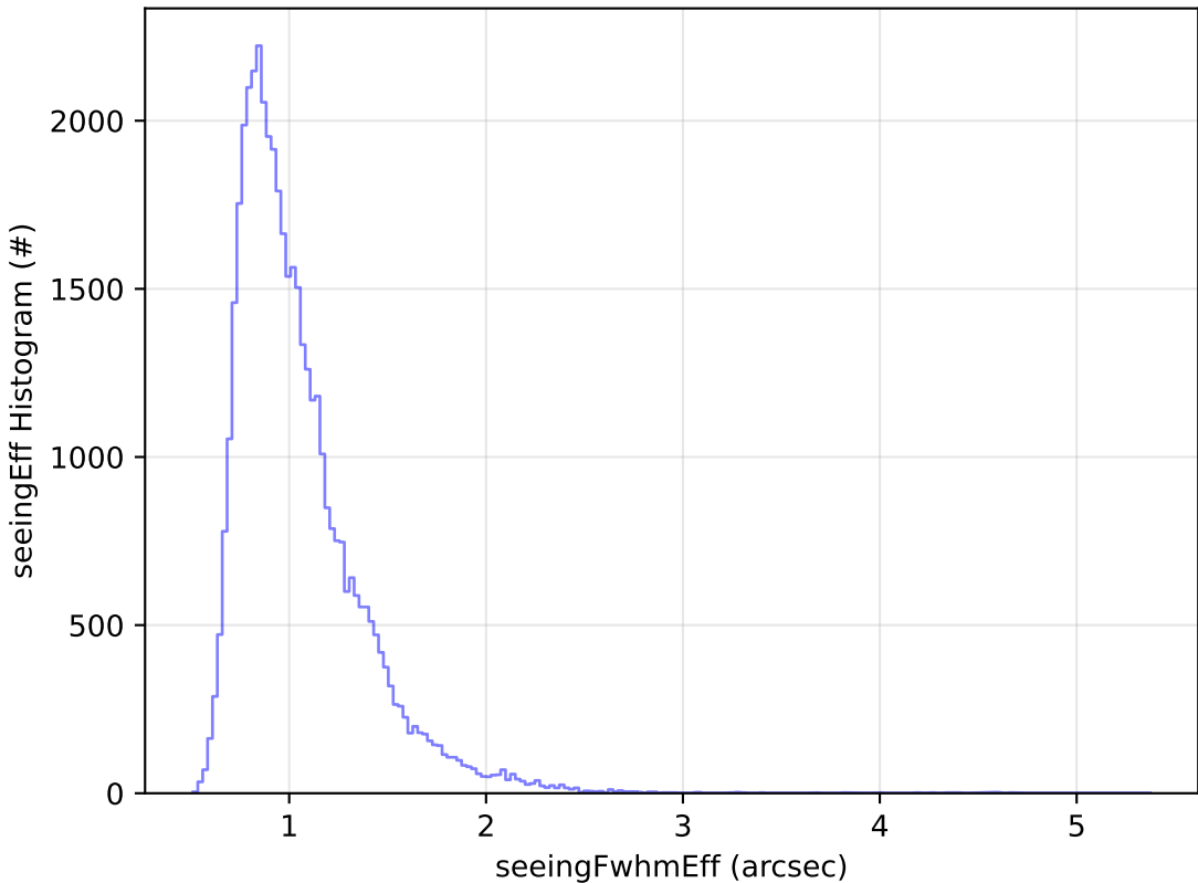
start_date_do90v3.4_10yrs Yr 1 z band: seeingEff Histogram
