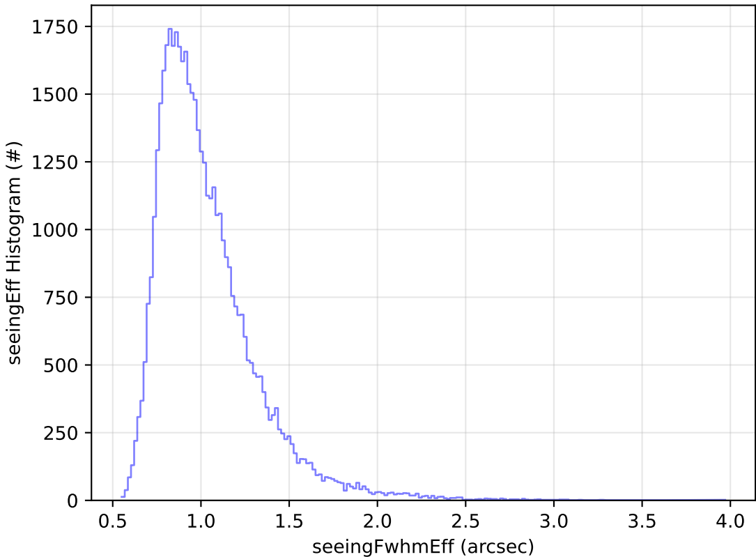
start_date_do90v3.4_10yrs Yr 1 y band: seeingEff Histogram
