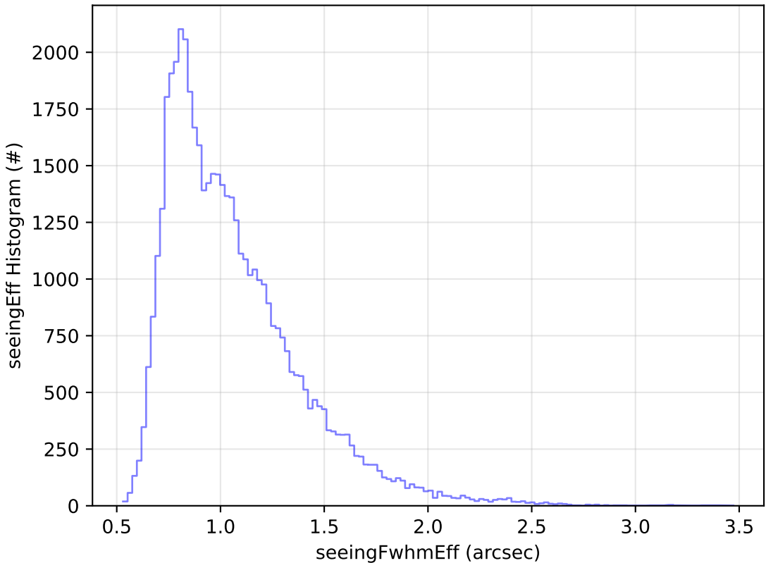
start_date_do90v3.4_10yrs Yr 1 r band: seeingEff Histogram
