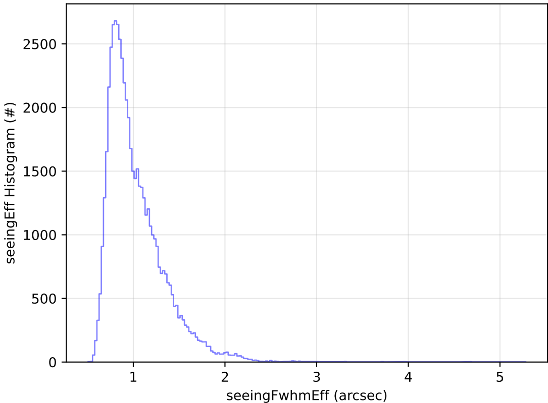
start_date_do90v3.4_10yrs Yr 1 i band: seeingEff Histogram
