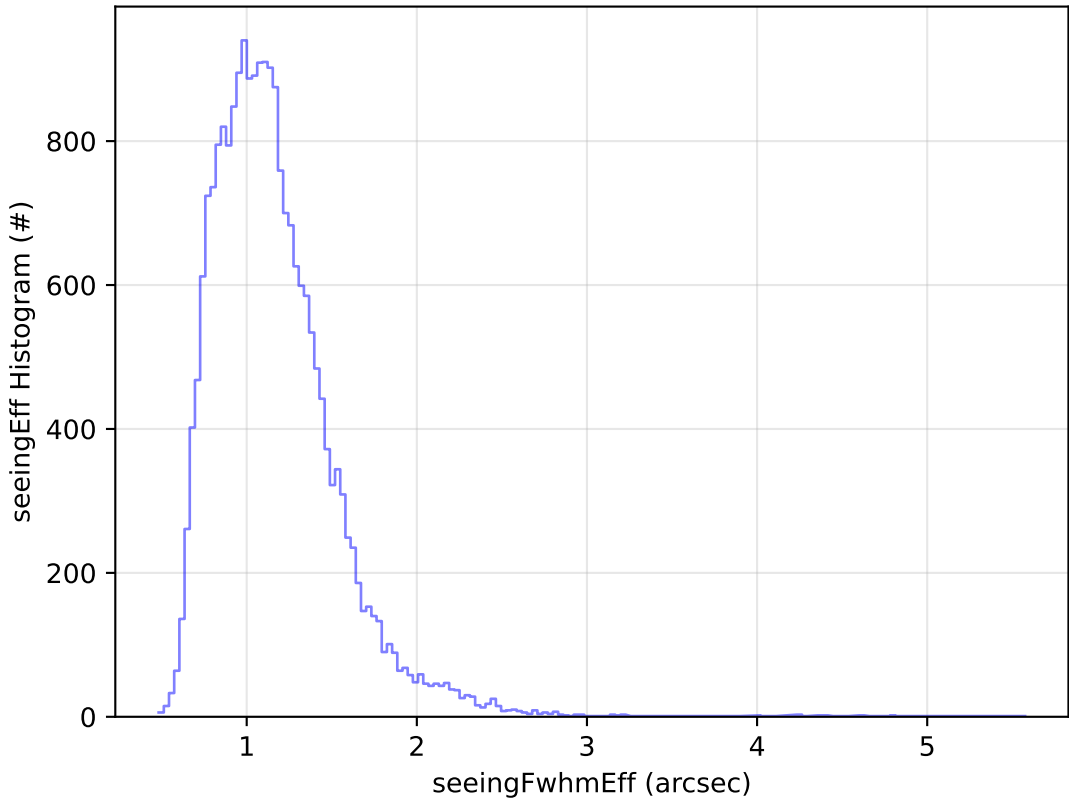
start_date_do90v3.4_10yrs Yr 1 g band: seeingEff Histogram
