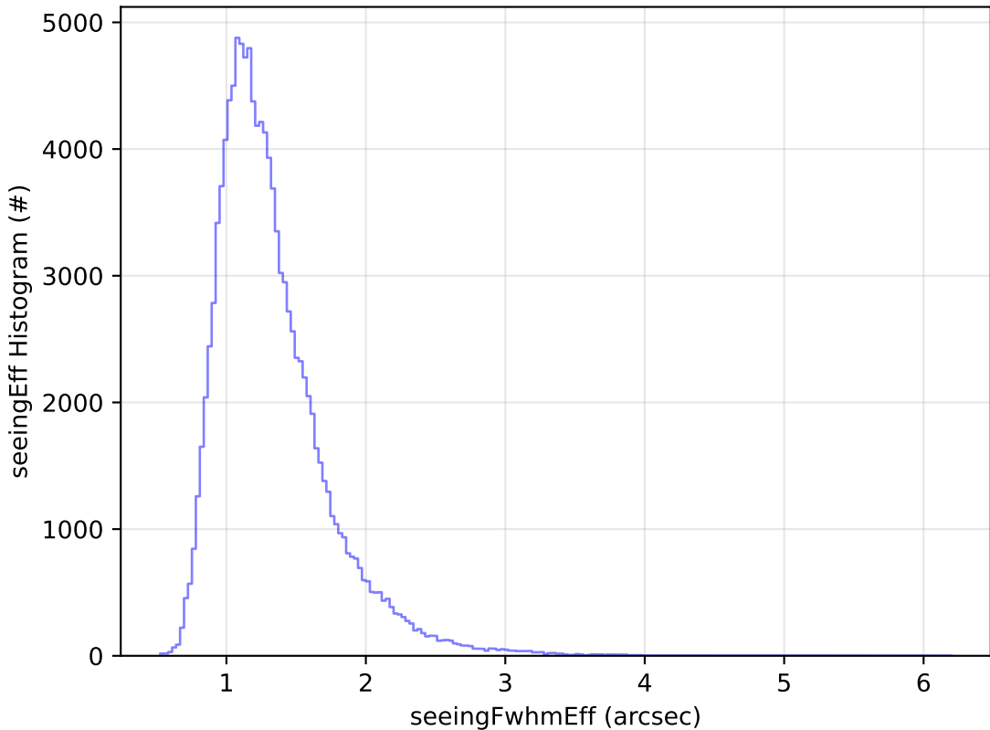
start_date_do90v3.4_10yrs WFD u band: seeingEff Histogram
