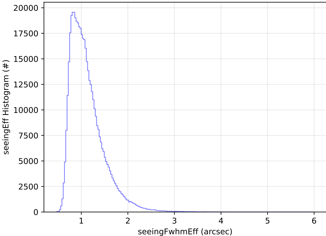
start_date_do90v3.4_10yrs WFD r band: seeingEff Histogram
