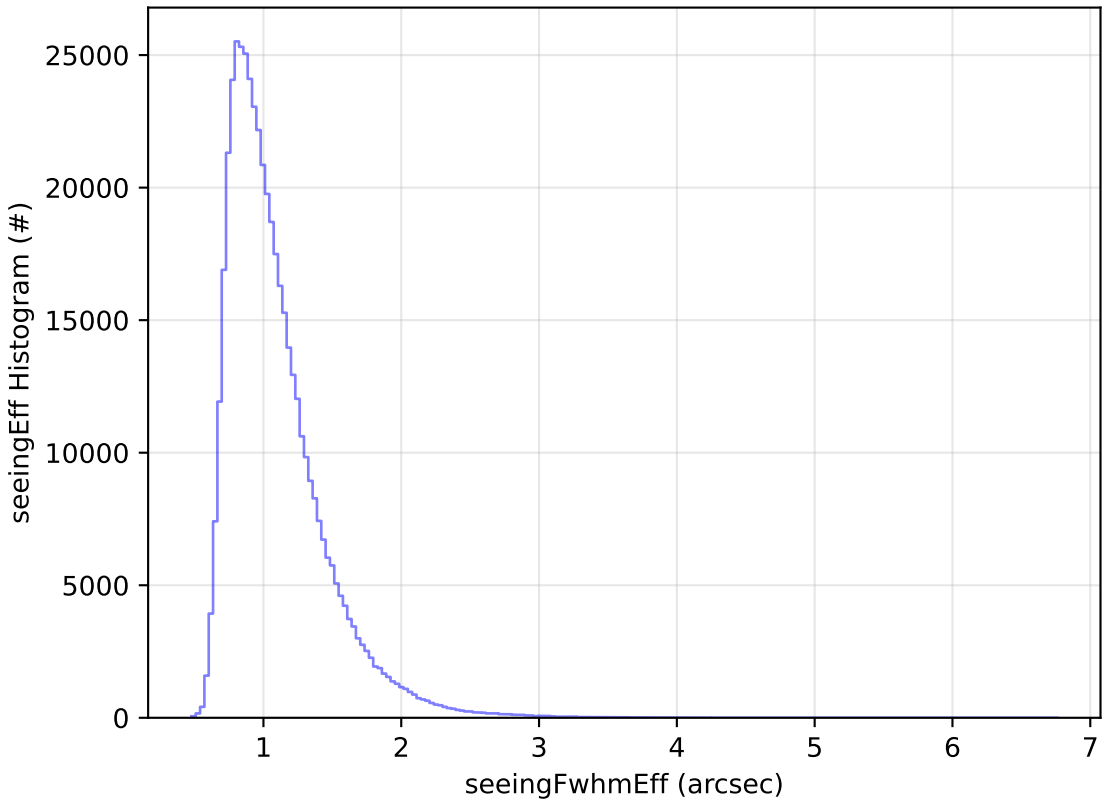
start_date_do90v3.4_10yrs WFD i band: seeingEff Histogram
