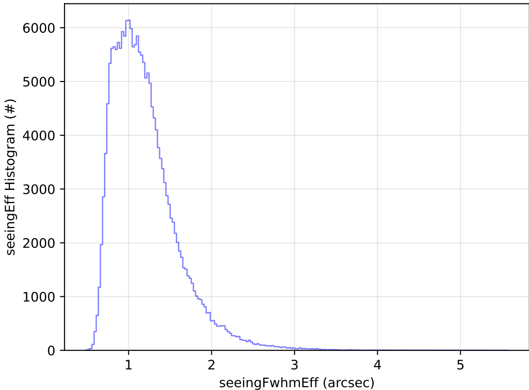
start_date_do90v3.4_10yrs WFD g band: seeingEff Histogram
