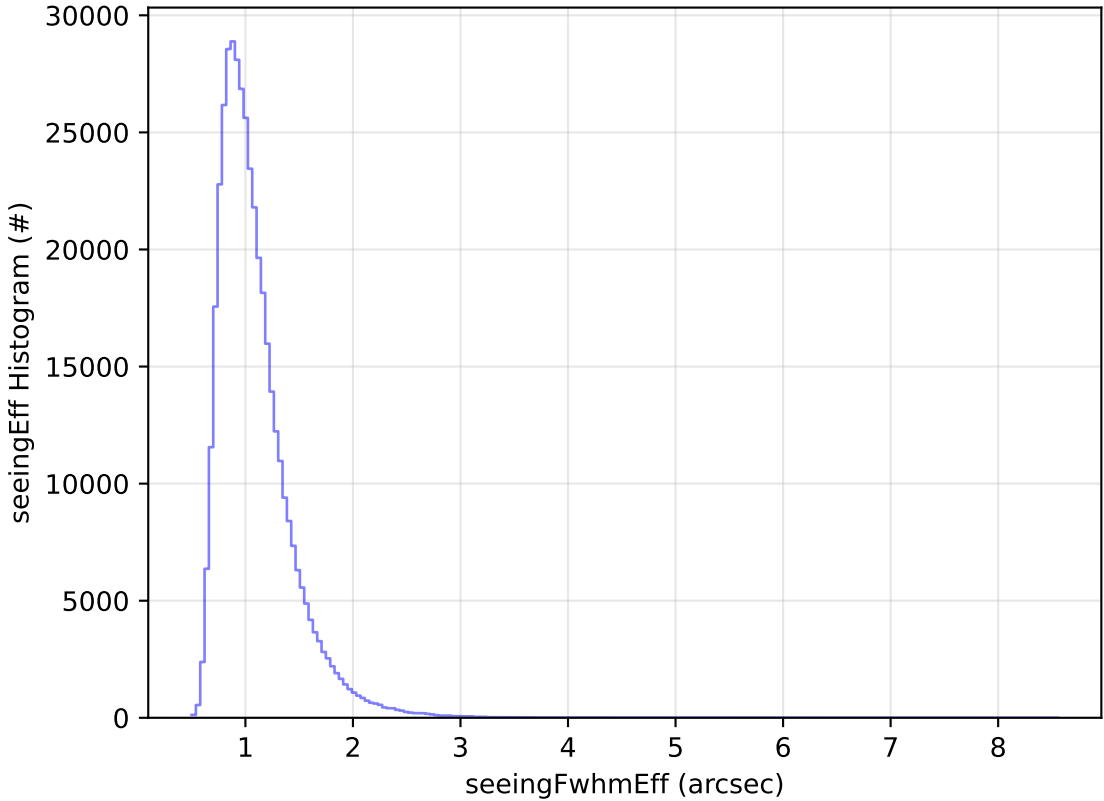
start_date_do90v3.4_10yrs All sky z band: seeingEff Histogram
