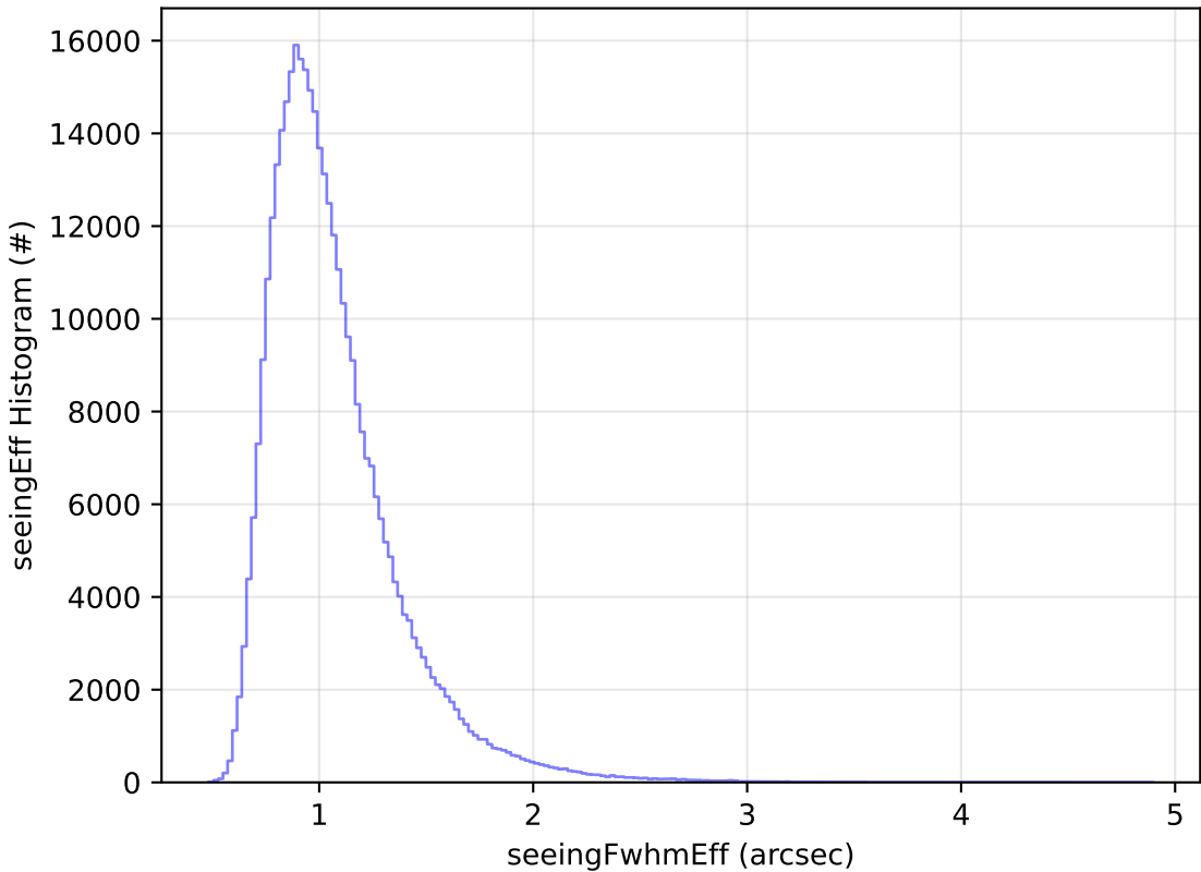
start_date_do90v3.4_10yrs All sky y band: seeingEff Histogram
