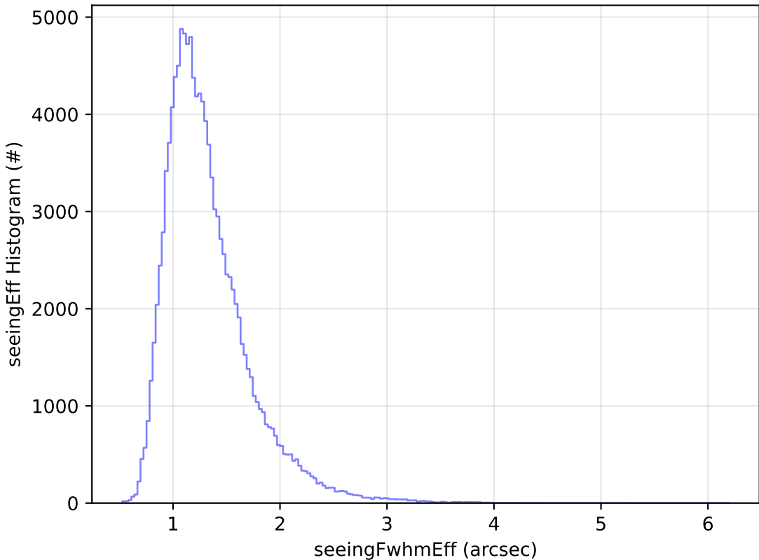
start_date_do90v3.4_10yrs All sky u band: seeingEff Histogram
