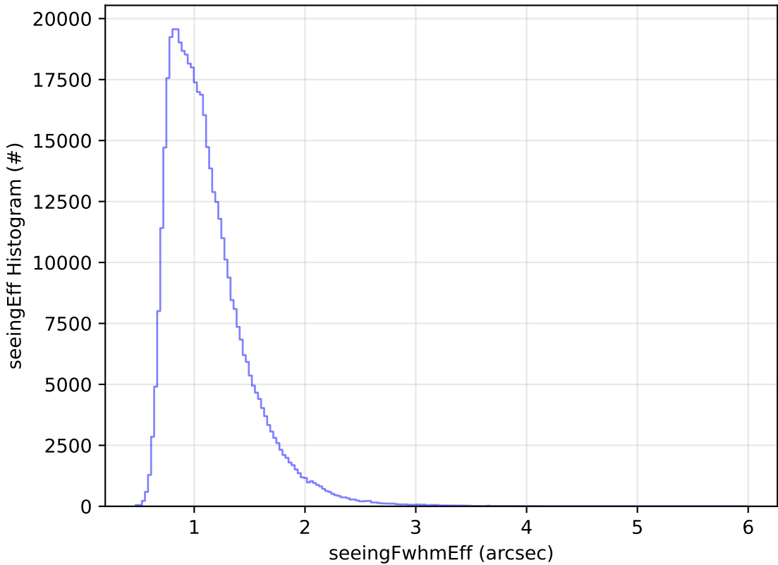
start_date_do90v3.4_10yrs All sky r band: seeingEff Histogram
