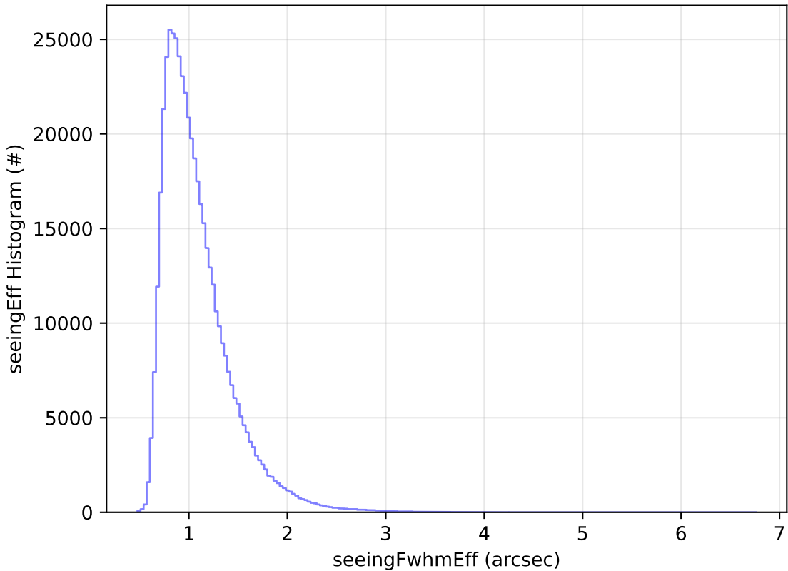
start_date_do90v3.4_10yrs All sky i band: seeingEff Histogram
