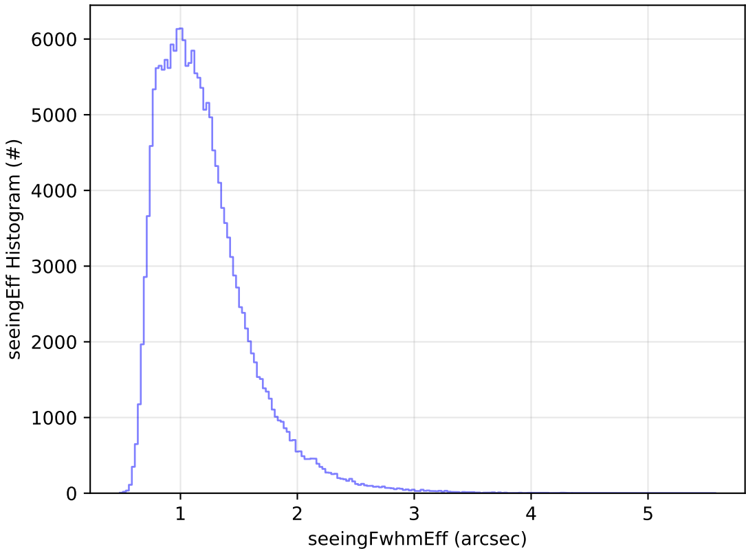
start_date_do90v3.4_10yrs All sky g band: seeingEff Histogram
