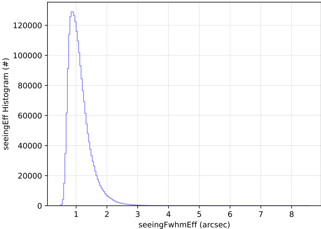
start_date_do90v3.4_10yrs All sky all bands: seeingEff Histogram
