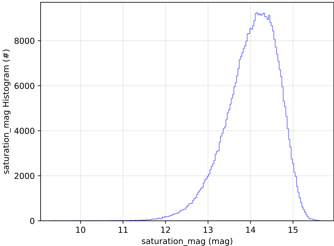
start_date_do90v3.4_10yrs WFD z band: saturation_mag Histogram
