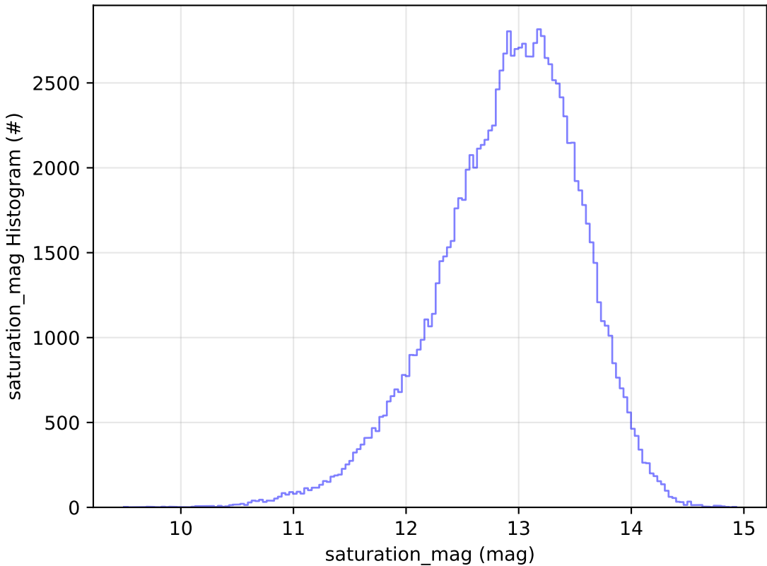
start_date_do90v3.4_10yrs WFD u band: saturation_mag Histogram
