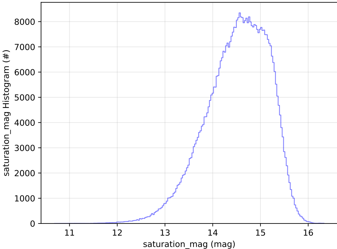
start_date_do90v3.4_10yrs WFD r band: saturation_mag Histogram
