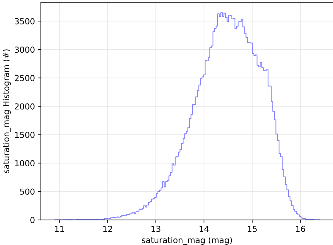
start_date_do90v3.4_10yrs WFD g band: saturation_mag Histogram
