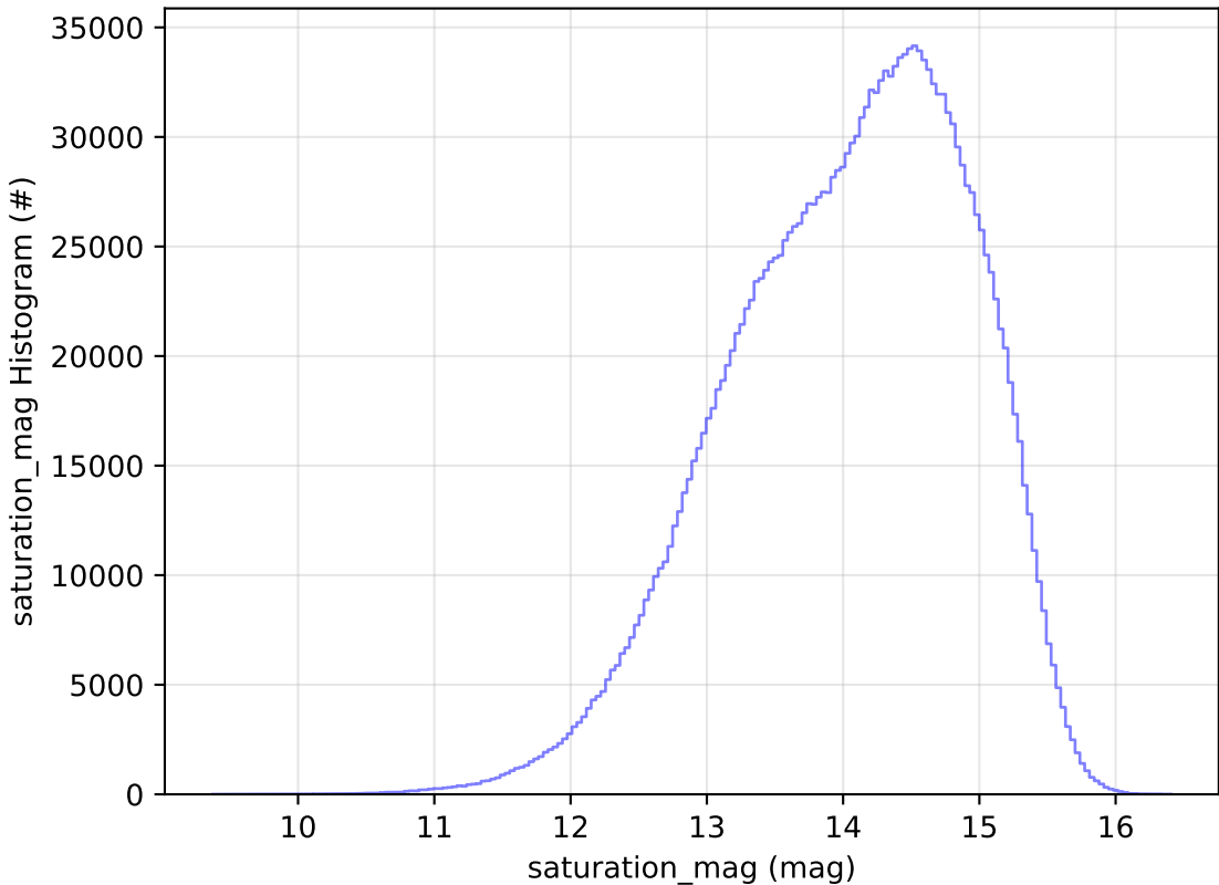
start_date_do90v3.4_10yrs WFD all bands: saturation_mag Histogram
