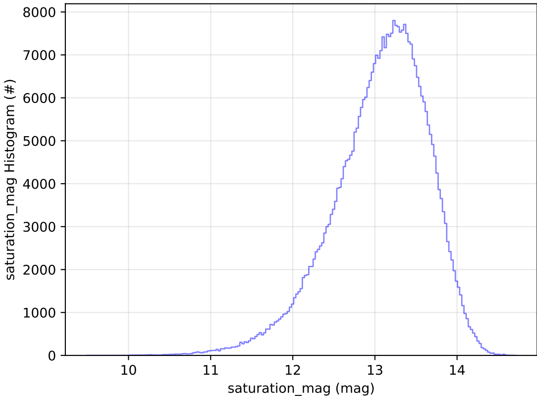
start_date_do90v3.4_10yrs All sky y band: saturation_mag Histogram
