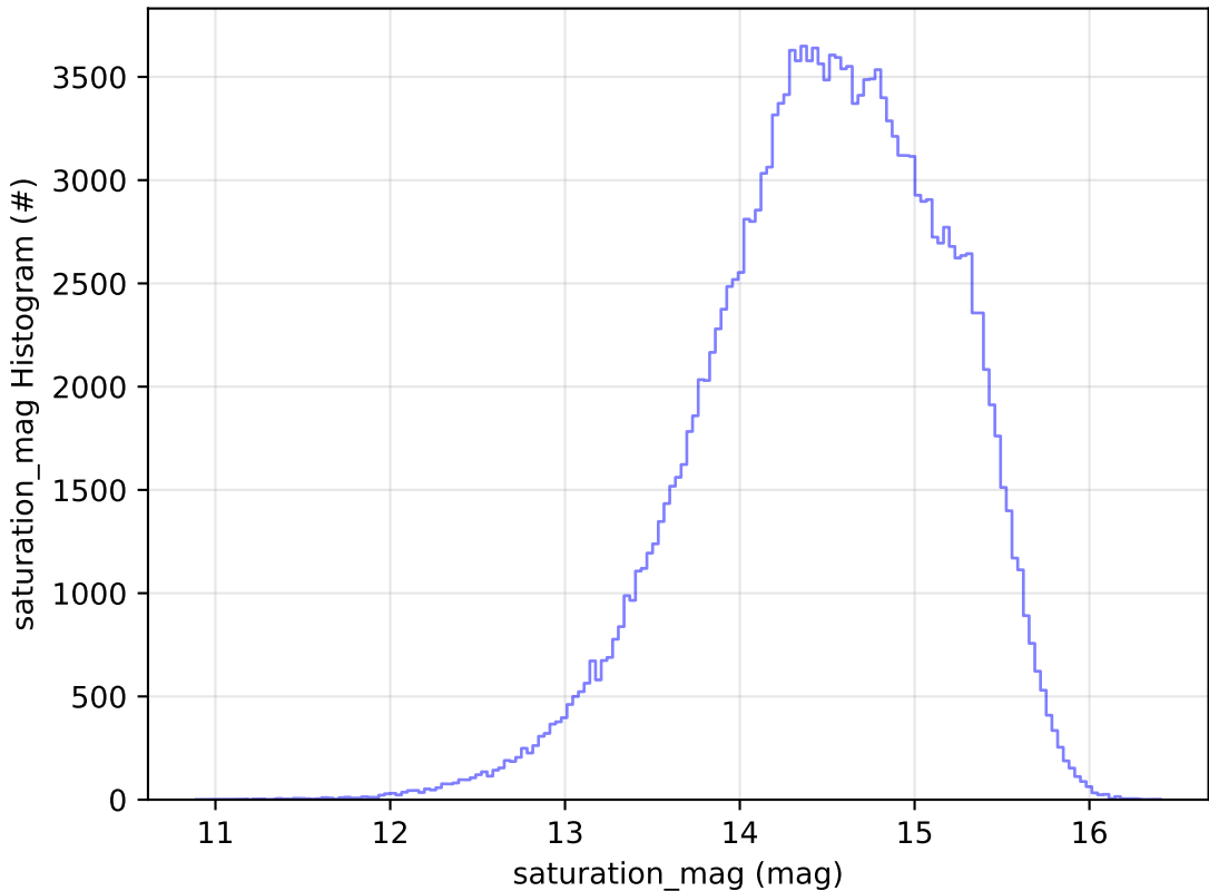
start_date_do90v3.4_10yrs All sky g band: saturation_mag Histogram
