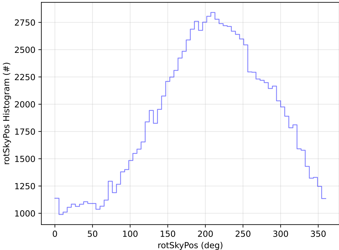
start_date_do90v3.4_10yrs WFD u band: rotSkyPos Histogram
