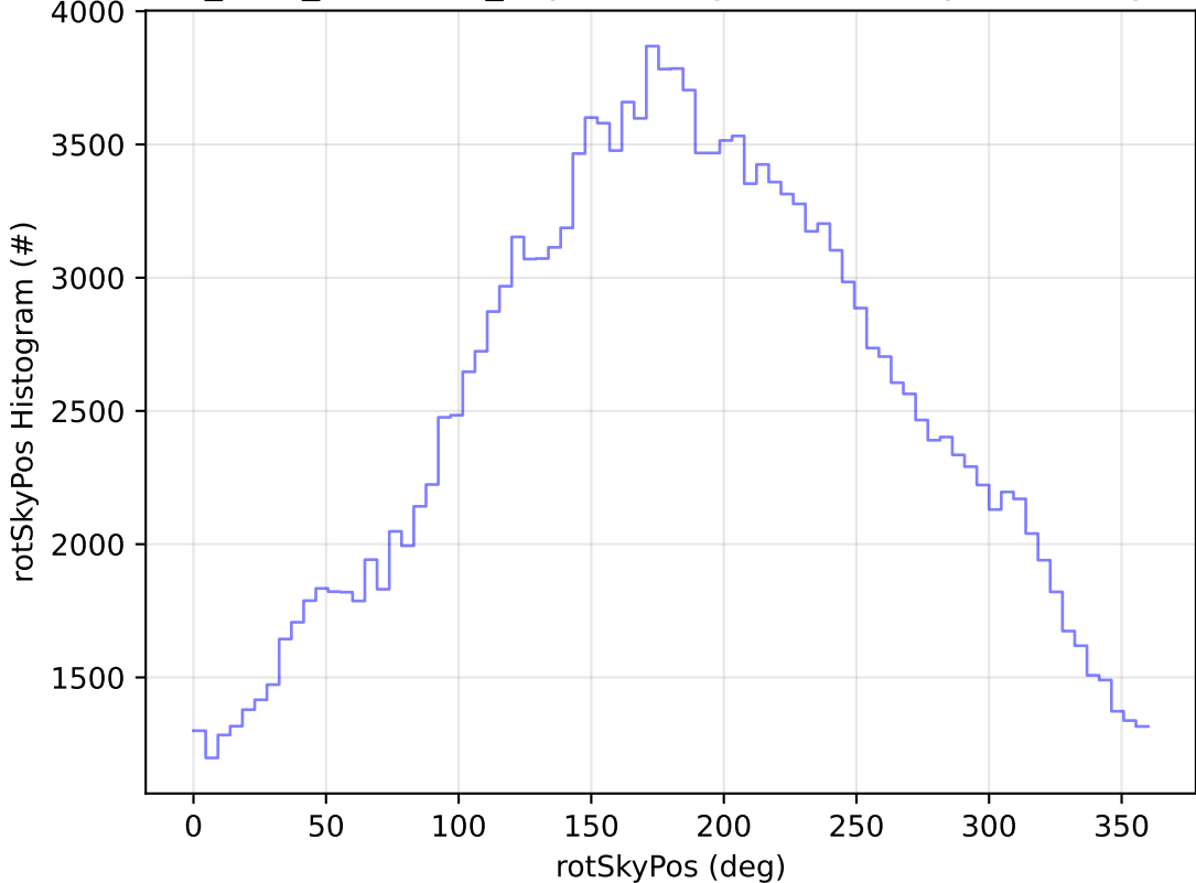
start_date_do90v3.4_10yrs WFD g band: rotSkyPos Histogram
