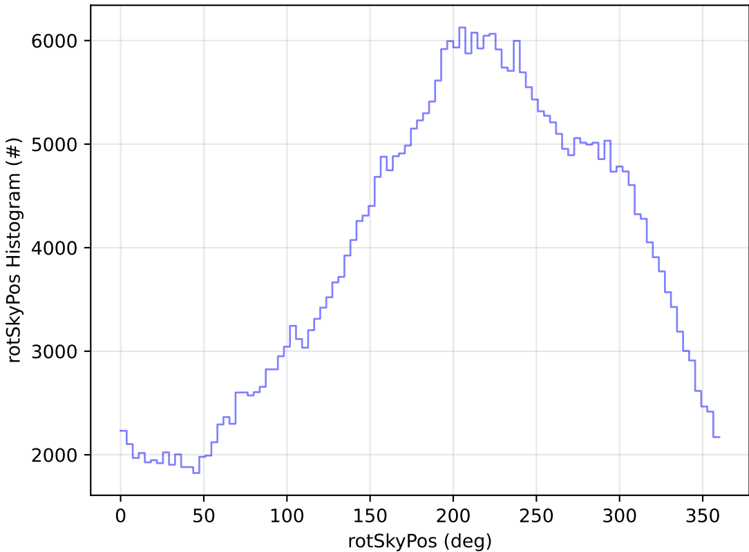
start_date_do90v3.4_10yrs All sky y band: rotSkyPos Histogram
