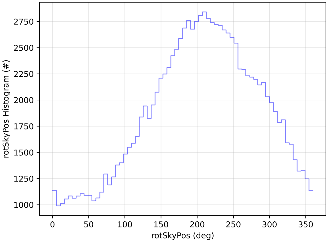
start_date_do90v3.4_10yrs All sky u band: rotSkyPos Histogram
