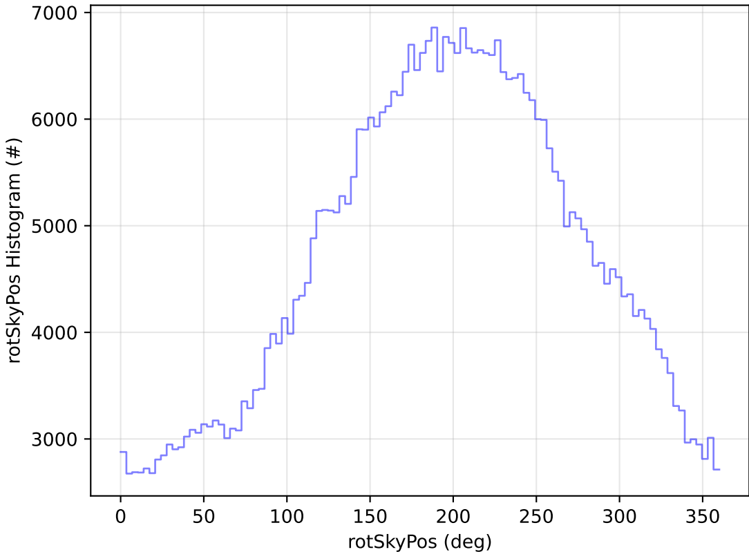
start_date_do90v3.4_10yrs All sky r band: rotSkyPos Histogram
