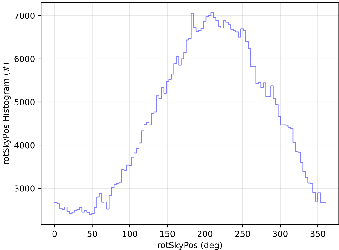
start_date_do90v3.4_10yrs All sky i band: rotSkyPos Histogram
