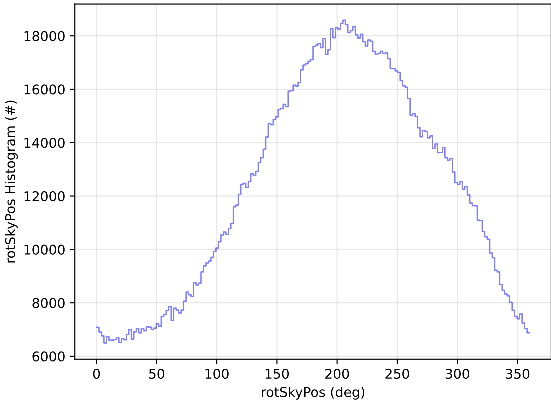
start_date_do90v3.4_10yrs All sky all bands: rotSkyPos Histogram
