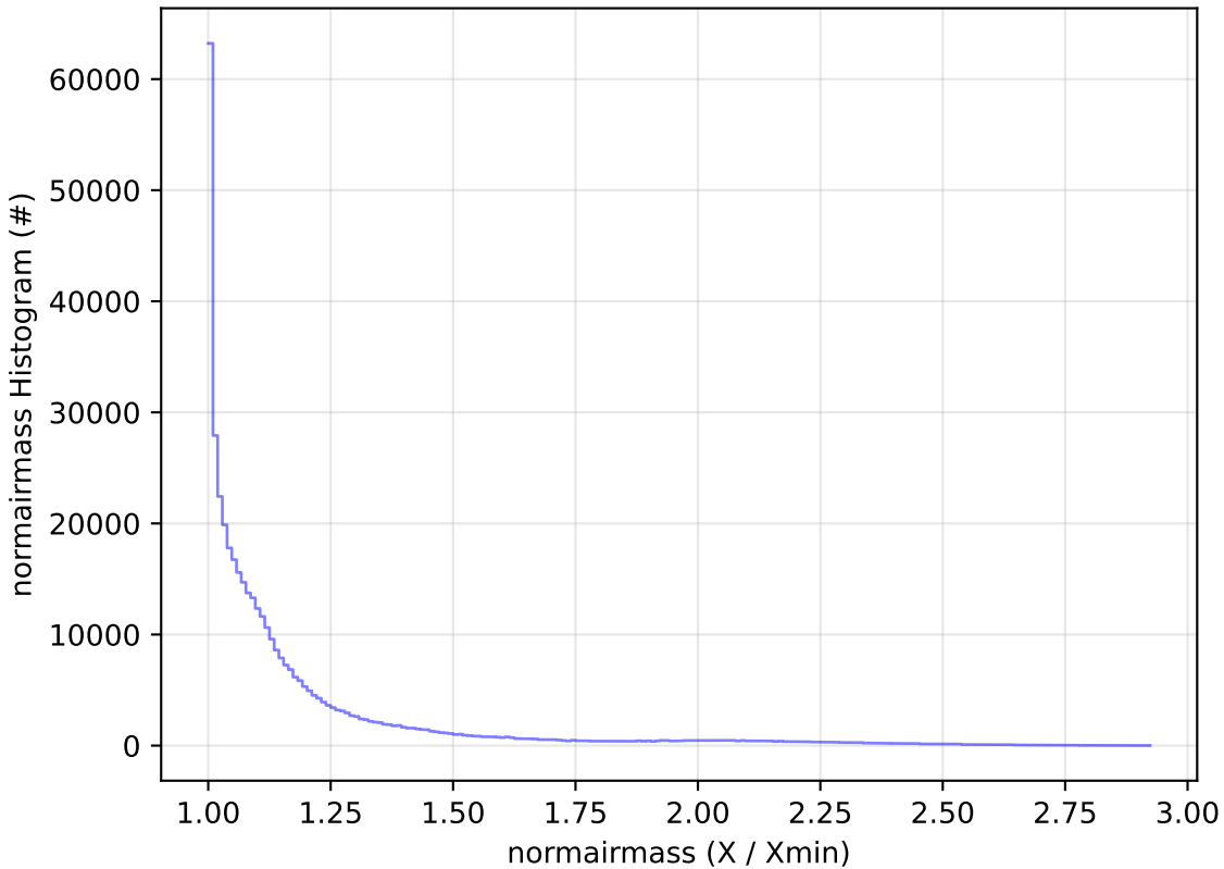
start_date_do90v3.4_10yrs WFD z band: normairmass Histogram
