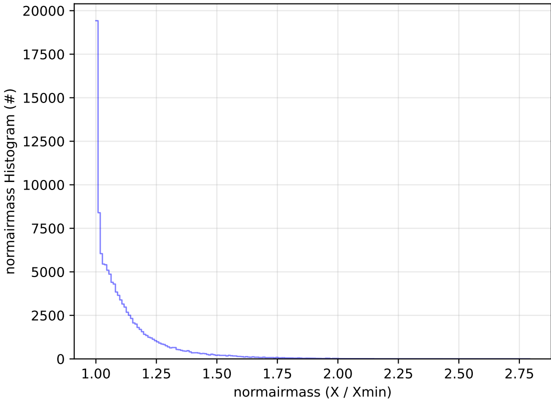
start_date_do90v3.4_10yrs WFD u band: normairmass Histogram
