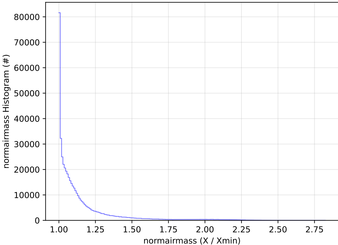
start_date_do90v3.4_10yrs WFD r band: normairmass Histogram
