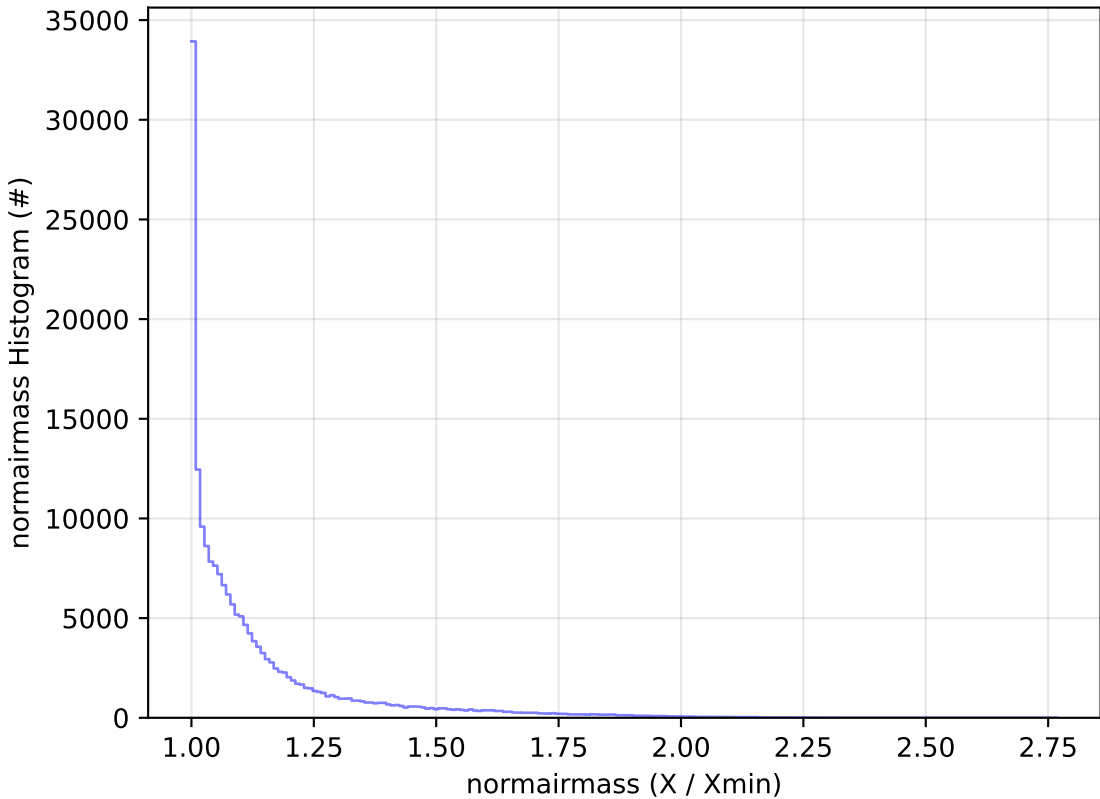
start_date_do90v3.4_10yrs WFD g band: normairmass Histogram
