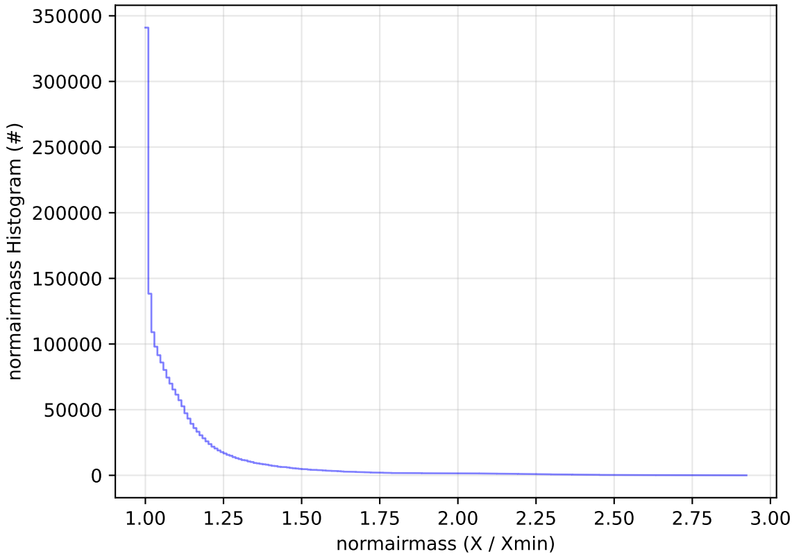
start_date_do90v3.4_10yrs WFD all bands: normairmass Histogram
