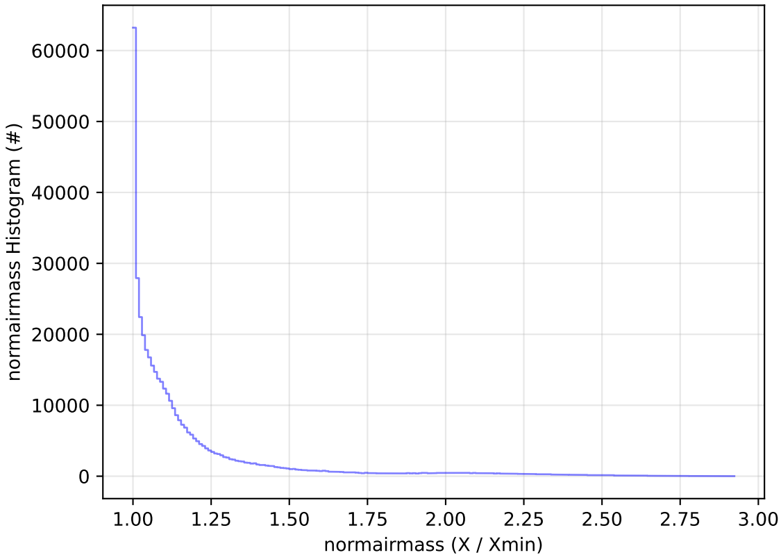
start_date_do90v3.4_10yrs All sky z band: normairmass Histogram
