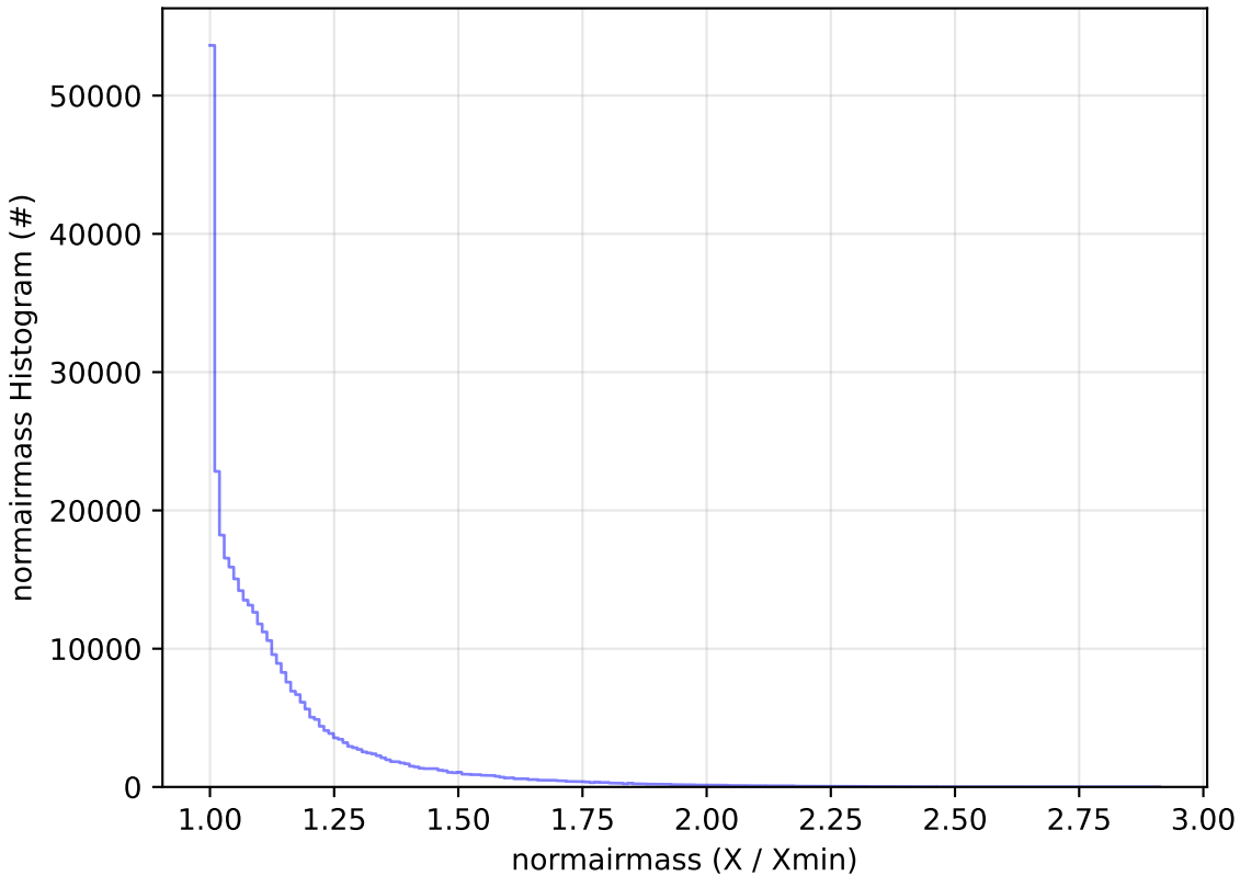
start_date_do90v3.4_10yrs All sky y band: normairmass Histogram
