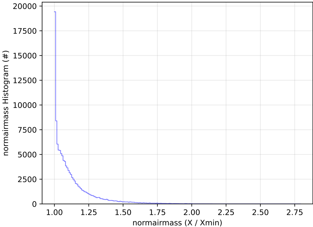
start_date_do90v3.4_10yrs All sky u band: normairmass Histogram
