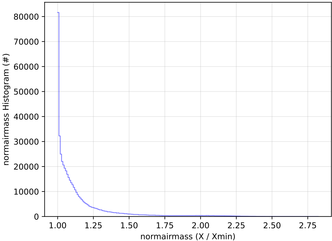
start_date_do90v3.4_10yrs All sky r band: normairmass Histogram
