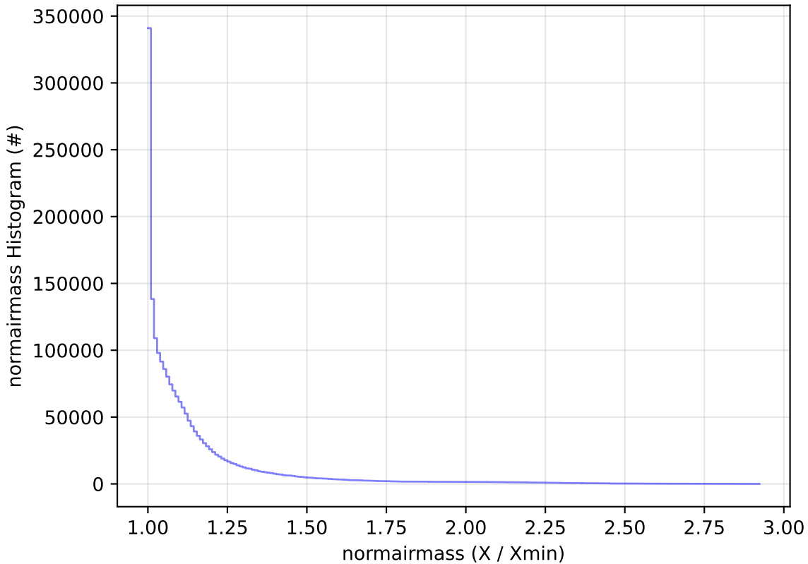
start_date_do90v3.4_10yrs All sky all bands: normairmass Histogram
