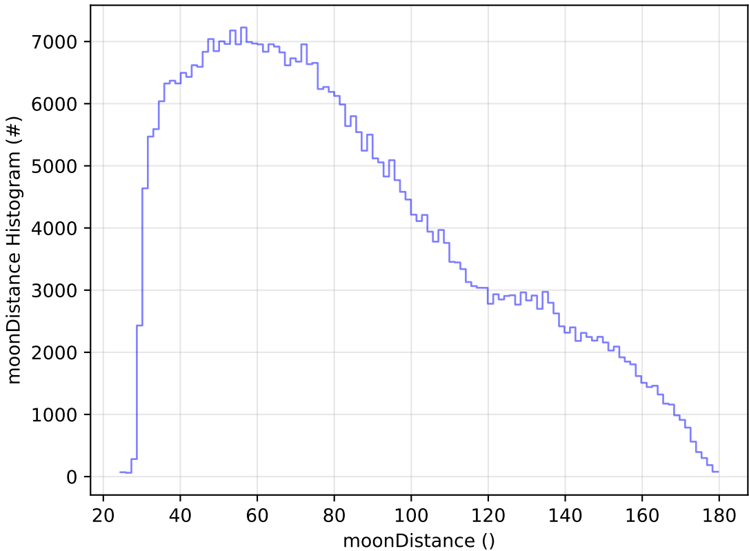
start_date_do90v3.4_10yrs WFD z band: moonDistance Histogram
