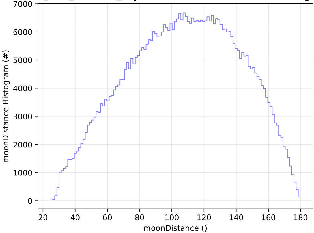
start_date_do90v3.4_10yrs WFD r band: moonDistance Histogram
