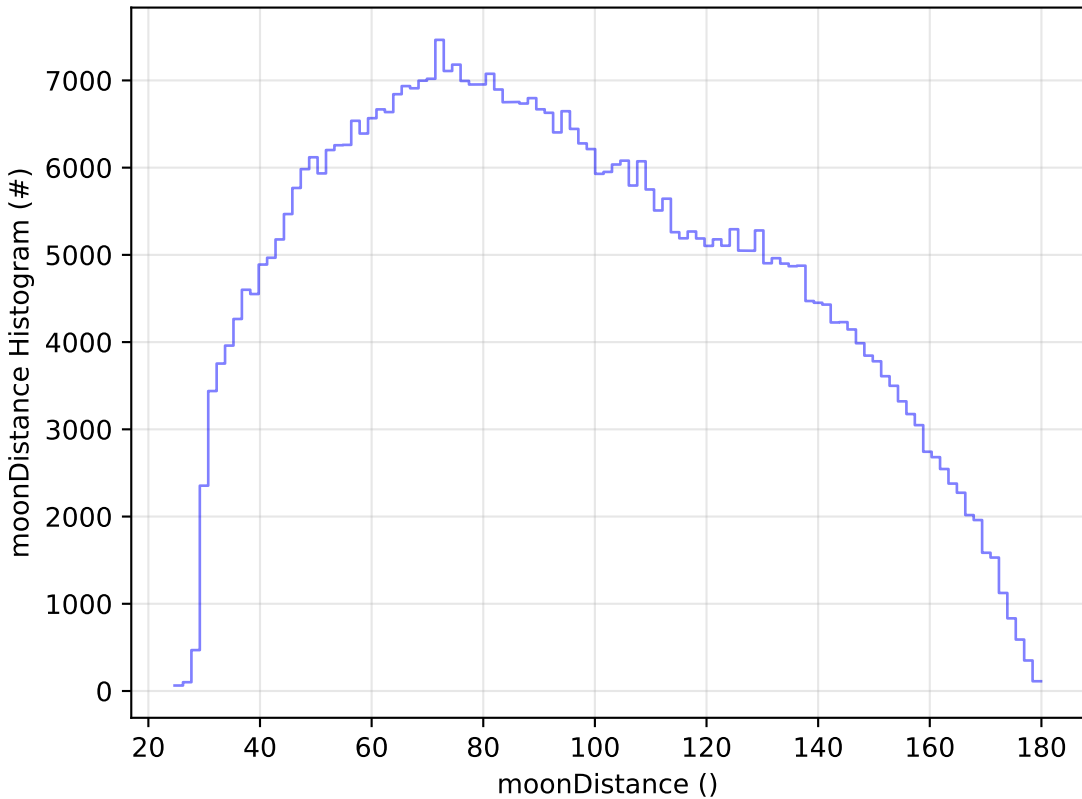
start_date_do90v3.4_10yrs WFD i band: moonDistance Histogram
