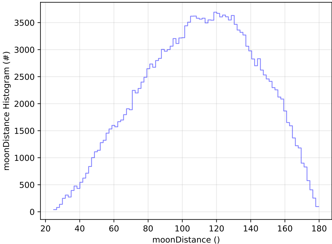
start_date_do90v3.4_10yrs WFD g band: moonDistance Histogram
