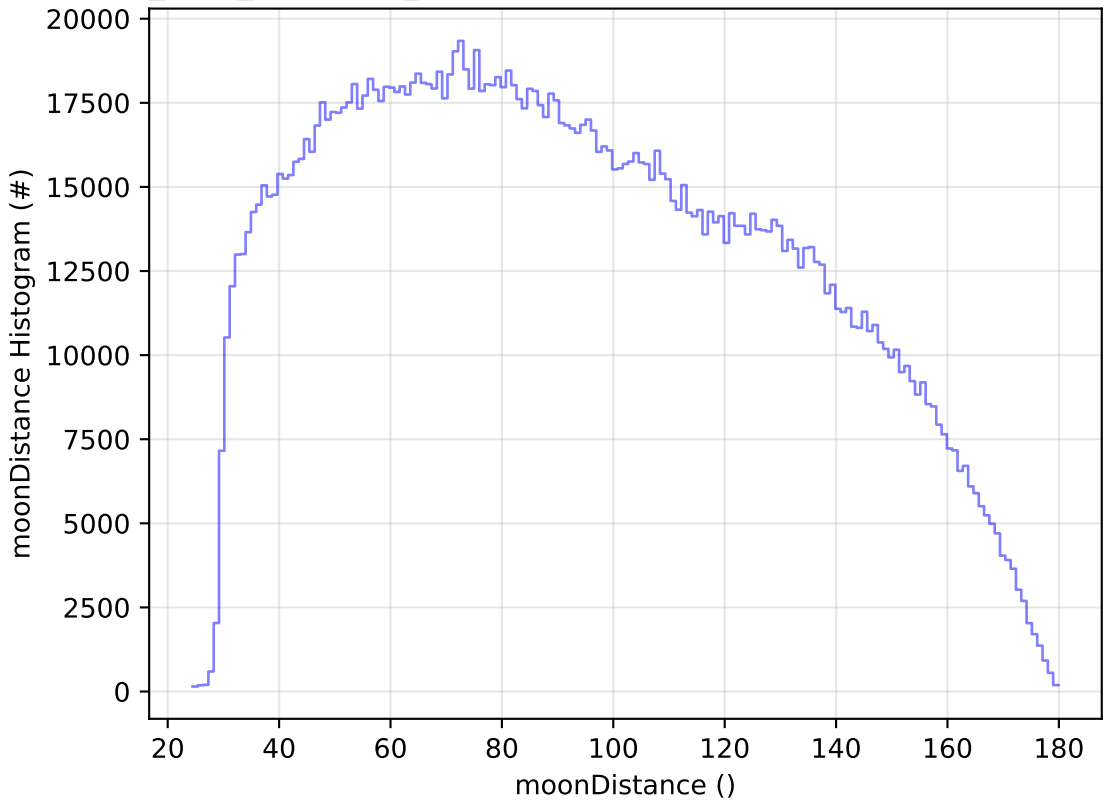
start_date_do90v3.4_10yrs WFD all bands: moonDistance Histogram
