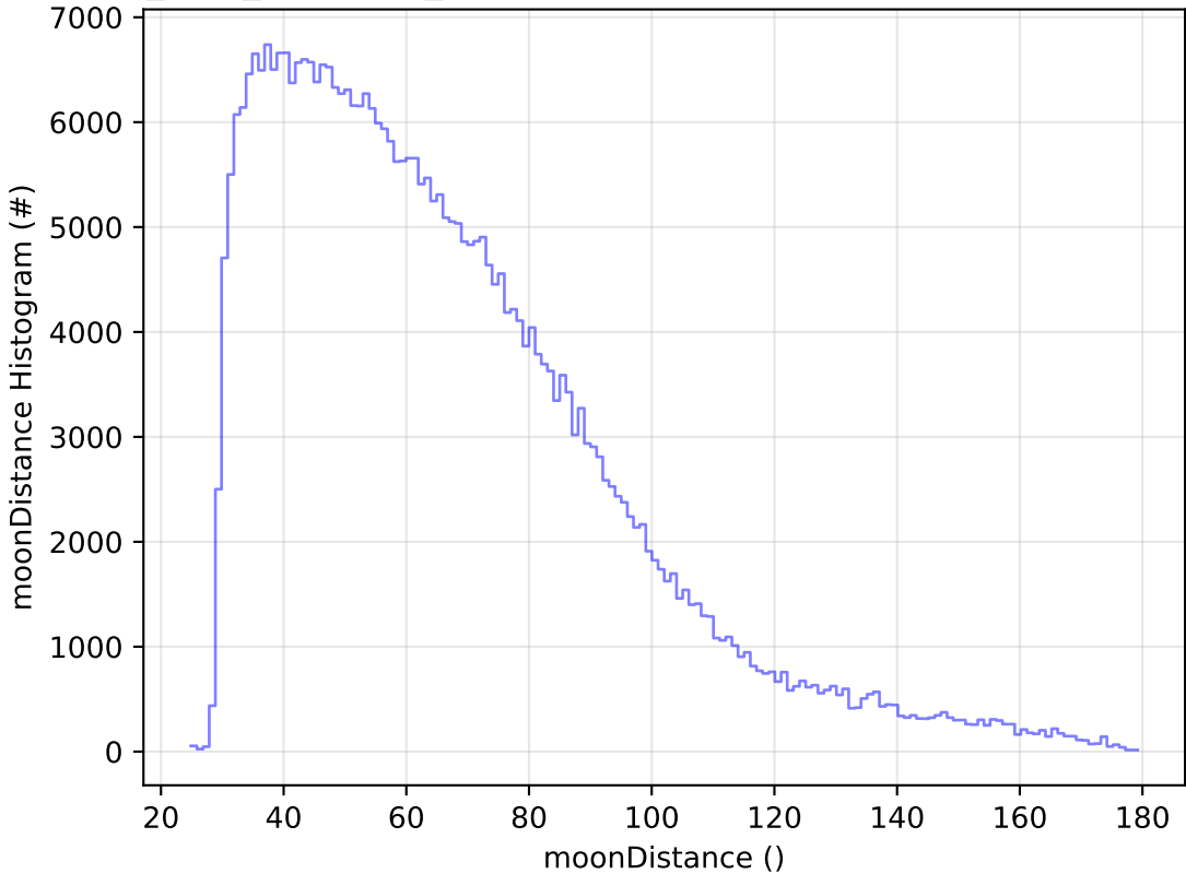
start_date_do90v3.4_10yrs All sky y band: moonDistance Histogram
