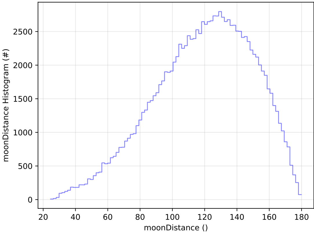
start_date_do90v3.4_10yrs All sky u band: moonDistance Histogram
