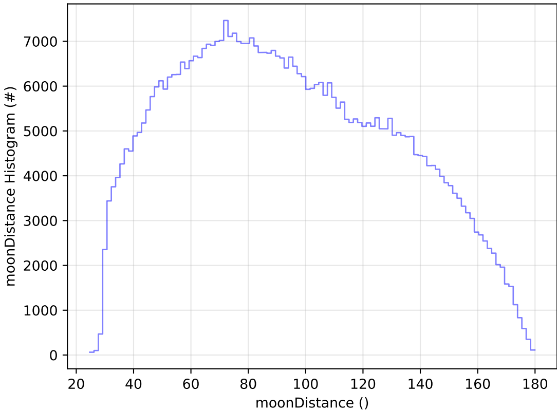
start_date_do90v3.4_10yrs All sky i band: moonDistance Histogram
